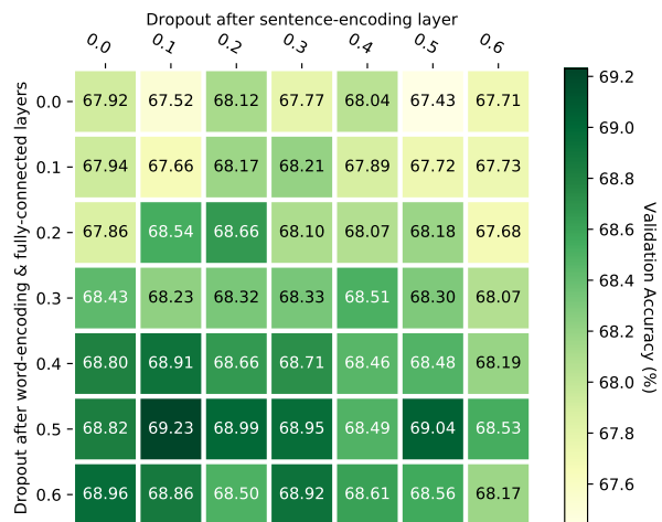
Figure 3: Dropout Ablation.
